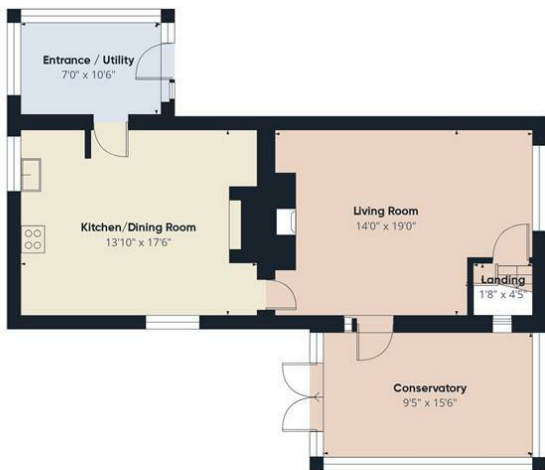
Floor 0 Building 1
